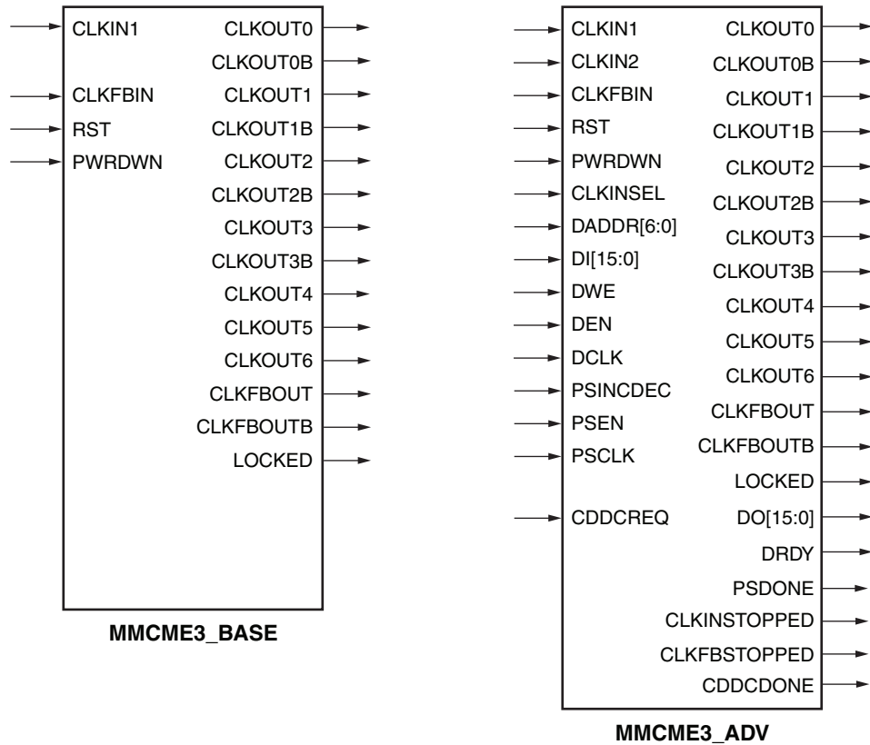
Figure 3-2: MMCM Primitives
