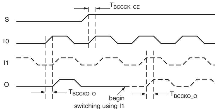
Figure 2-10: BUFGMUX Timing Diagram
