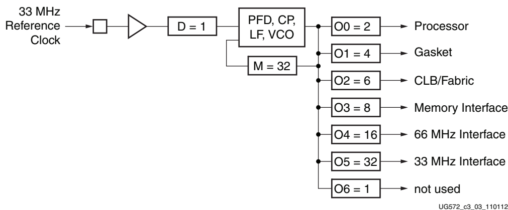
Figure 3-3: MMCM as a Frequency Synthesizer
