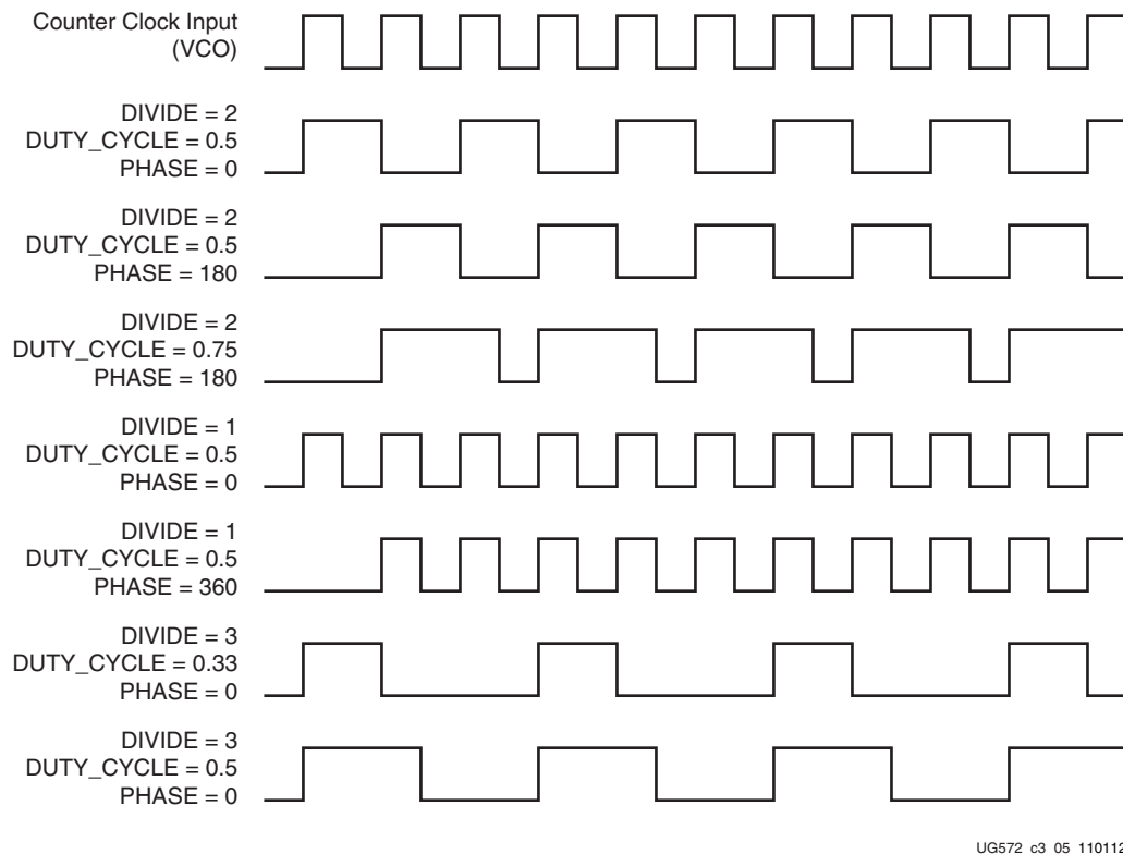
Figure 3-6: Output Counter Clock Synthesis Examples
