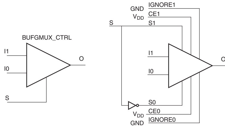
Figure 2-12: BUFGMUX_CTRL as BUFGCTRL
