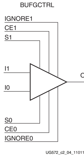
Figure 2-5: BUFGCTRL Primitive
