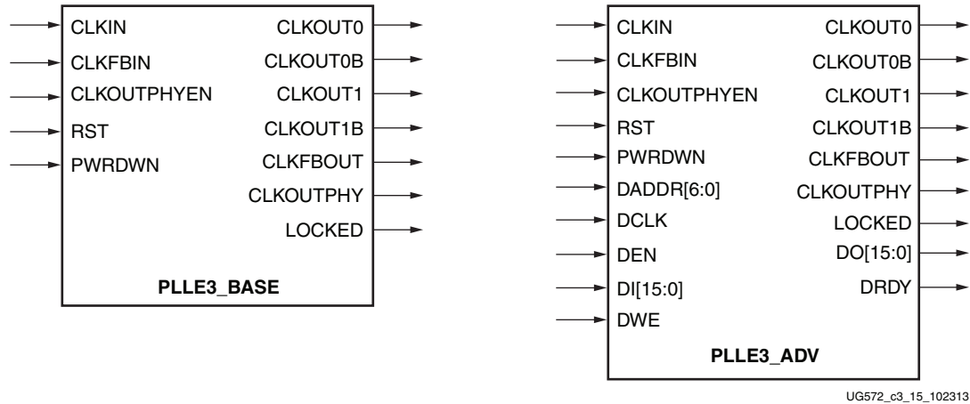
Figure 3-16: PLLE3_BASE and PLLE3_ADV
