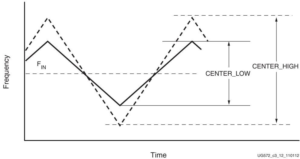
Figure 3-13: Center-Spread Modulation (CENTER_LOW vs. CENTER_HIGH)
