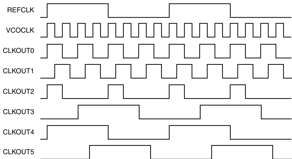
Figure 3-15: Example Waveform
