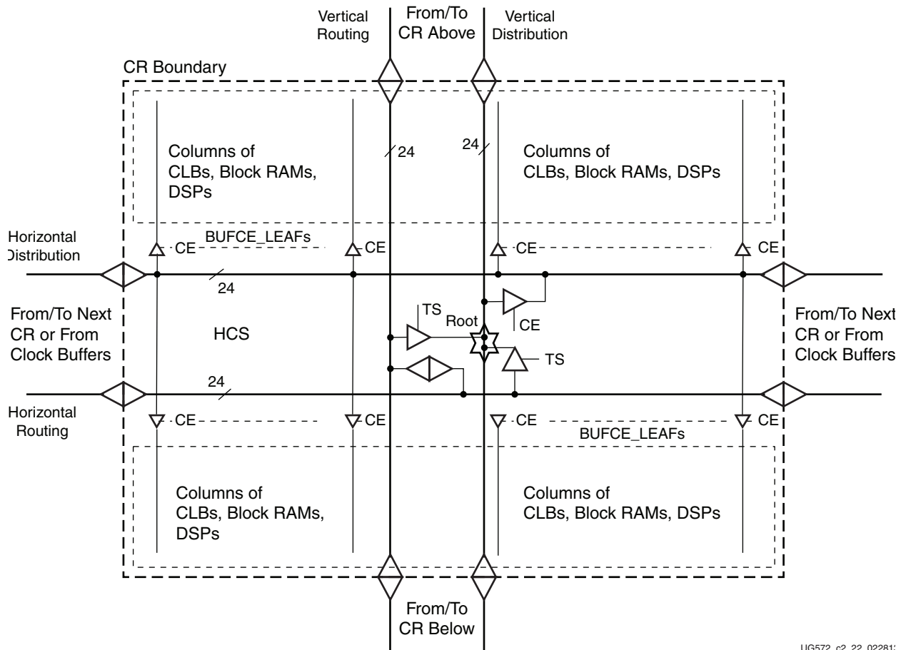
Figure 2-3: Clock Region Clcking
