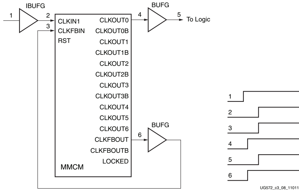
Figure 3-9: Global Clock Network Deskew Using Two BUFs
