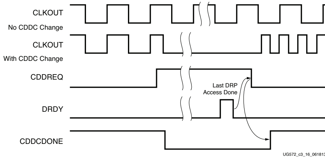
Figure 3-5: CDDC Timing Diagram
