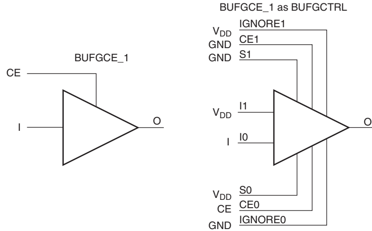
Figure 2-7: BUFGE_1 as BUFCTRL
