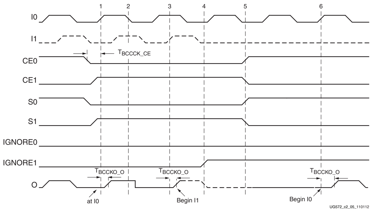
Figure 2-6: BUFGCTRL Timing Diagram
