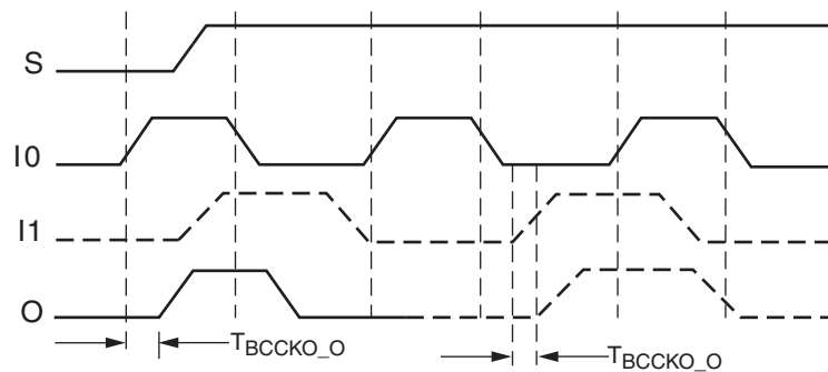
Figure 2-13: BUFGMUX_CTRL Timing Diagram
