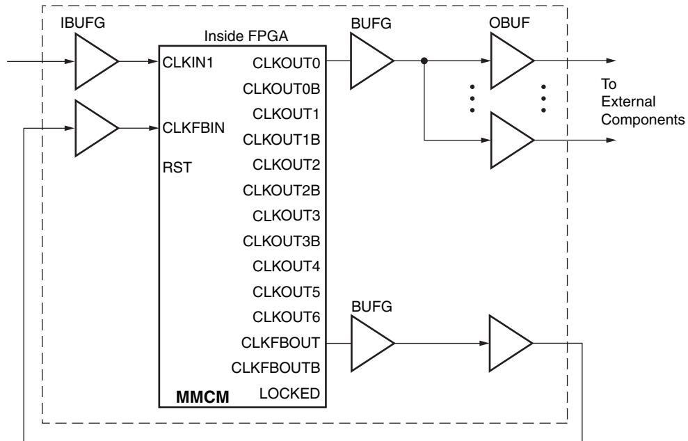
Figure 3-11: Zero Delay Buffer
