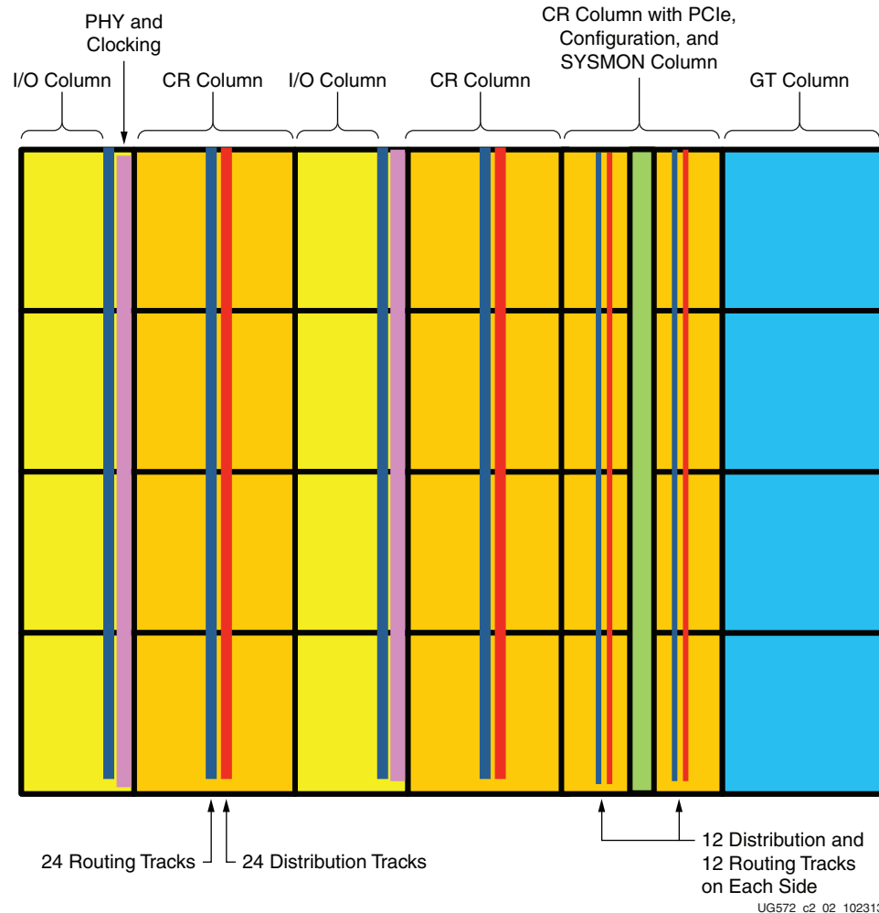
Figure 2-2: Vertical Clocking
