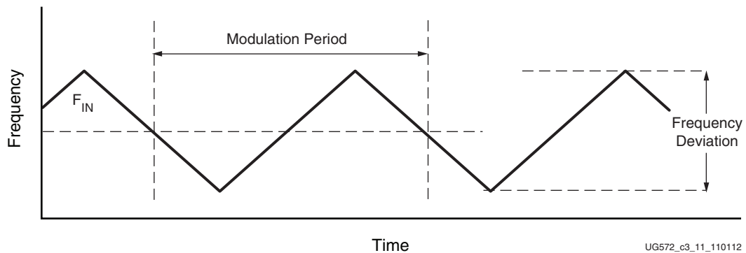
Figure 3-12: Center-Spread Modulation
