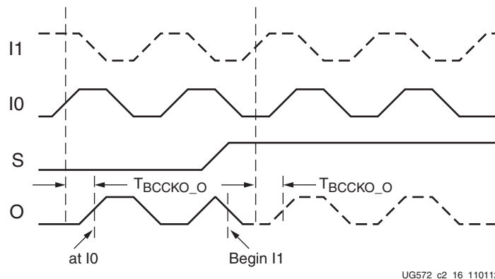
Figure 2-15: Asynchronous MUX Timing Diagram
