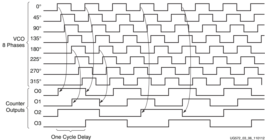
Figure 3-7: Selecting VCO Phases
