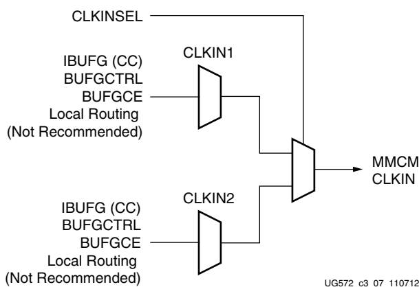
Figure 3-8: Input Clock Switching
