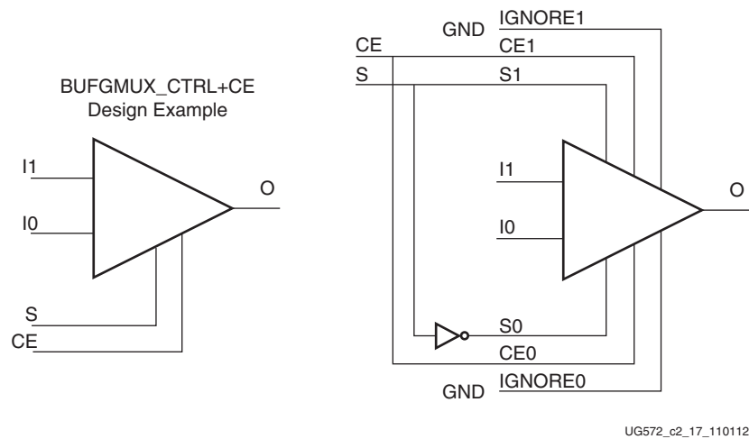
Figure 2-16: BUFGMUX_CTRL with a CE and BUFGCTRL
