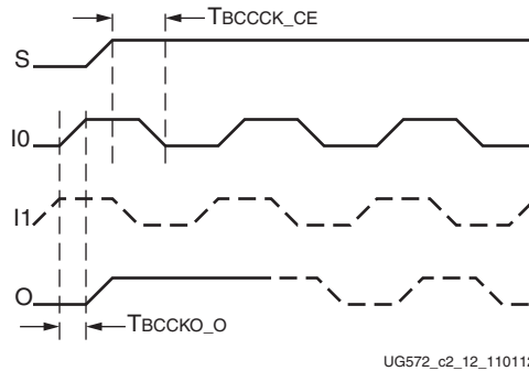
Figure 2-11: BUFGMUX_1 Timing Diagram
