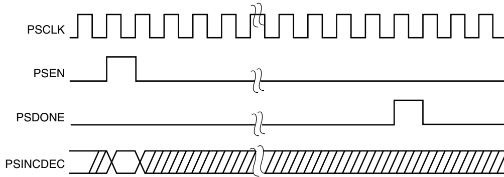
Figure 3-4: Phase Shift Timing Diagram
