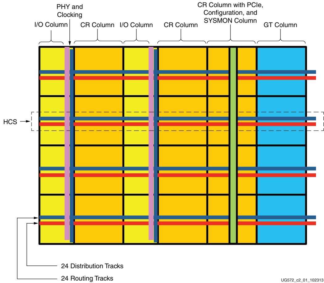
Figure 2-1: Horizontal Clocking
