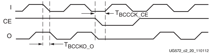
Figure 2-19: BUFGCE Timing Diagram
