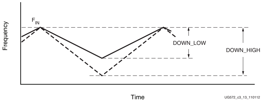
Figure 3-14: Down-Spread Modulation
