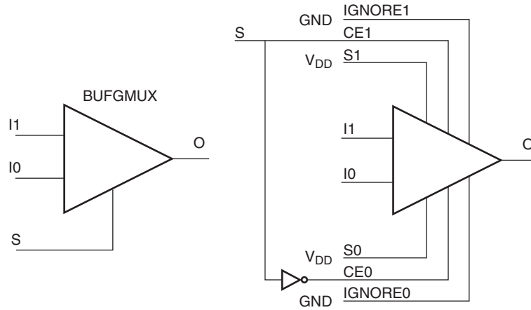
Figure 2-9: BUFGMUX as BUFGCTRL
