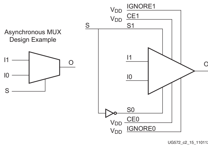
Figure 2-14: Asynchronous MUX with BUFCTRL Design Example
