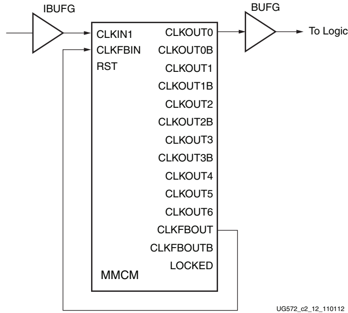
Figure 3-10: MMCM with Internal Feedback
